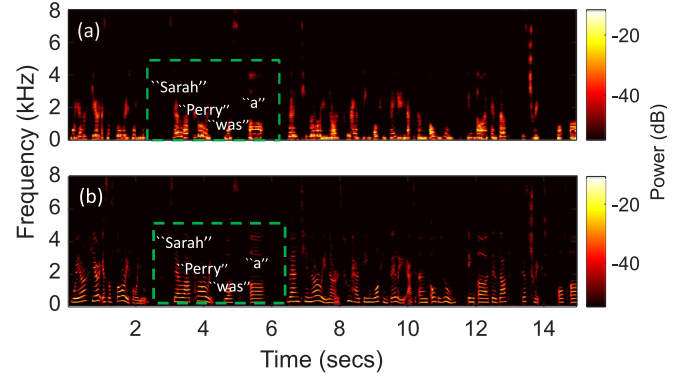
Figure 9: Spectrograms of (a) microphone-detected signal and (b) reconstructed voice signal. The vital voice information (refer to the annotated formants) are reconstructed by the Wave-Net. (Training loss = 0.00604357, Test loss = 0.00599584)
