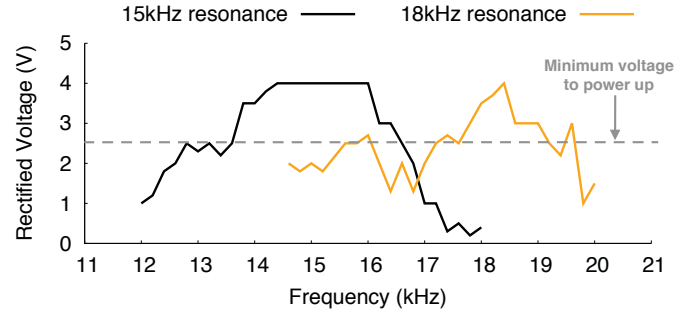
Figure 3—Recto-piezo. The figure plots the rectified voltage as a function of the downlink transmit frequency for two different recto-piezo configurations. One of the recto-piezos (in black) is electrically matched at 15 kHz and the second (in orange) at 18 kHz.
