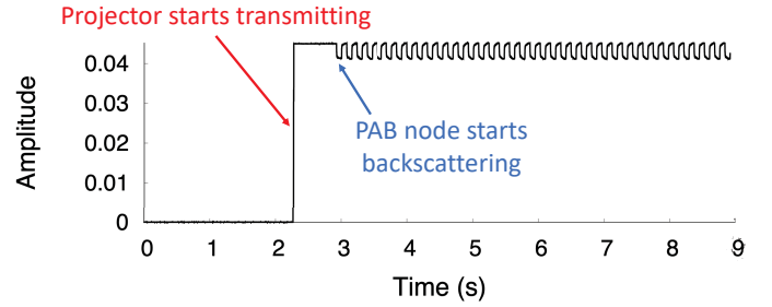
Figure 2—Received and Demodulated Backscatter Signal. The figure plots the received signal after demodulation and low-pass filtering. After PAB starts backscattering, the larger amplitude corresponds to the reflected state while the smaller amplitude corresponds to the non-reflected state. The node switches between these two states to communicate bits of 0s and 1s (using FM0 encoding).
