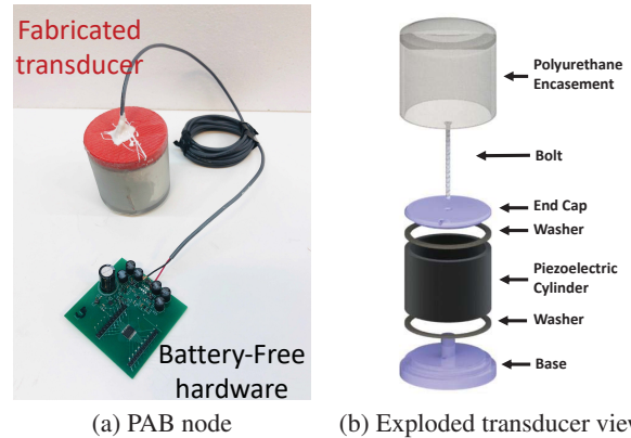
Figure 4—Mechanical and Hardware Fabrication. (a) shows the mechanically fabricated transducer with the battery-free analog-digital hardware design, (b) shows the exploded transducer view.
