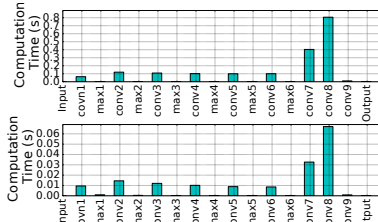
Fig. 7: The computation latency of YOLOv2’s layers on the edge (top) and cloud (bottom) respectively.
