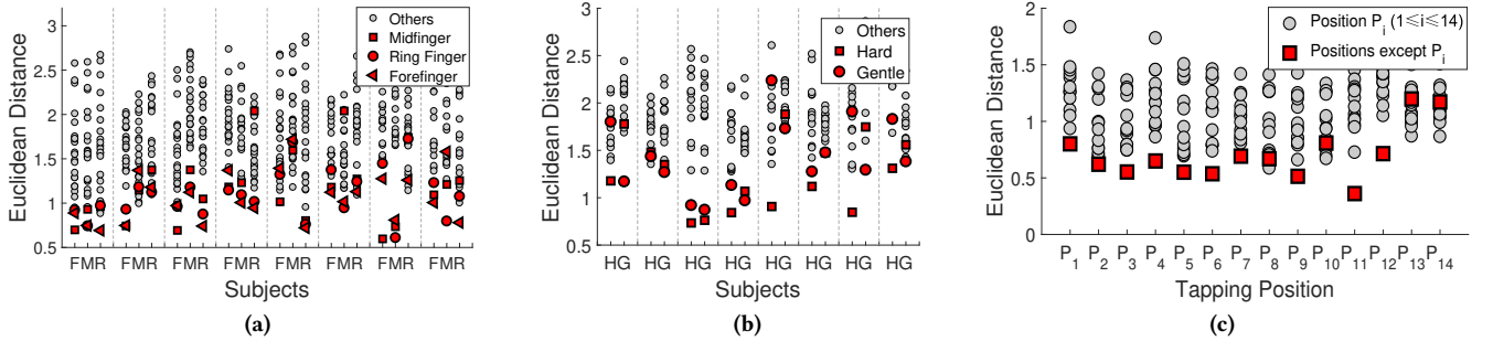
Figure 4: The Euclidean distance of samples generated by different (a) fingers, (b) tap strengths, and (c) locations.
