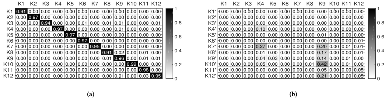
Figure 10: Confusion matrix of 12 keys, where (a) both the training and test samples are from the legitimate users (b) the training samples are from the legitimate users while the test samples are from the attackers.
