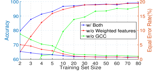
Figure 13: Impact of initial training set size.
