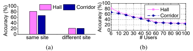
Figure 1: The accuracy of WIWHO drops significantly if the model is not tuned for the target environment (a), and if the number of target users is more than a dozen (b).
