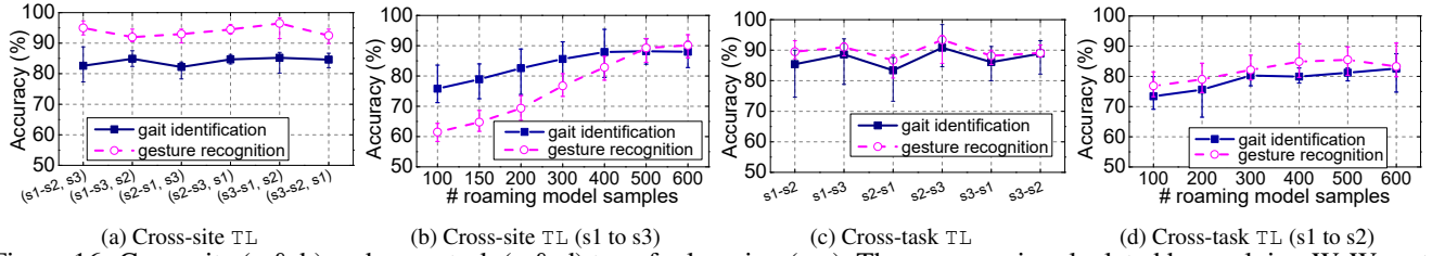
Figure 16: Cross-site (a & b) and cross-task (c & d) transfer learning (TL). The accuracy is calculated by applying W1WHO to six users and WIAG to six gestures. TL significantly reduces the number of samples required to learn a new roaming model.
