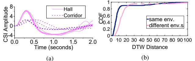
Figure 2: The CSI patterns for the same person from two different environments are different.
