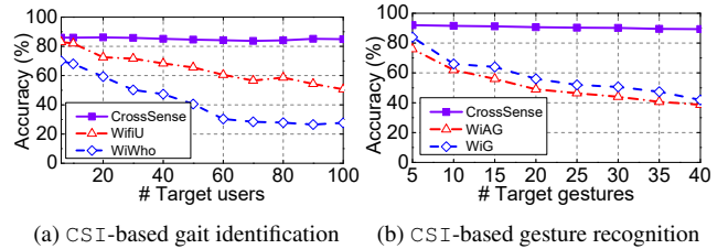
Figure 13: CSI-based sensing performance with different numbers of target activities. CROSSSENSE provides consistently good performance regardless of the problem size.
