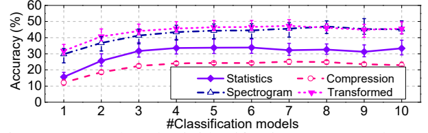
Figure 21: CSI-based gait identification accuracy when using different numbers of expert models to target 100 users.
