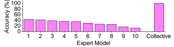
Figure 6: Percentages of samples that can be correctly classified by an expert on our expert model testing dataset.
