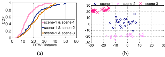
Figure 8: DTW distances of gait measurements for the same person increase if the samples are collected from different environments (a). The measurements of one user can be grouped into three clusters on a 2-d PCA space, each corresponds to where the data are gathered (b).
