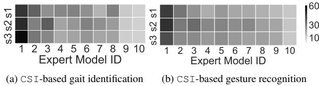
Figure 12: How often (as percentages) an expert model in Table 3 correctly classifies an input across sites (s1, s2, s3).
