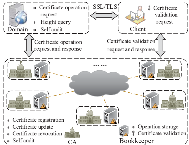
Fig. 1. Framework of CertChain
