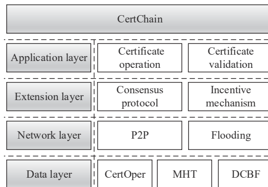
Fig. 2. Architecture of CertChain
