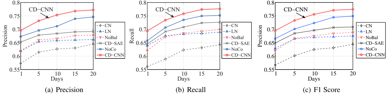
Figure 2: Classification with varying data collecting days.
