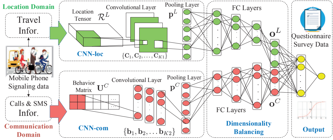
Figure 1: The framework of CD-CNN.
