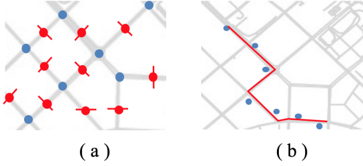
Fig. 4. Pre-Processing. (a) a glimpse of new road network after re-segments. New segment points are marked with ticks. (b) an example of map-matching. Red line respects a trajectory mapped to a route on the road network which connecting GPS points.
