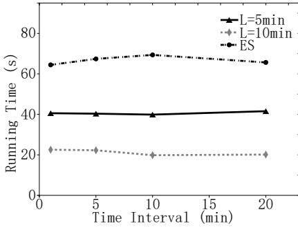
Fig. 16. Processing time over different time intervals
