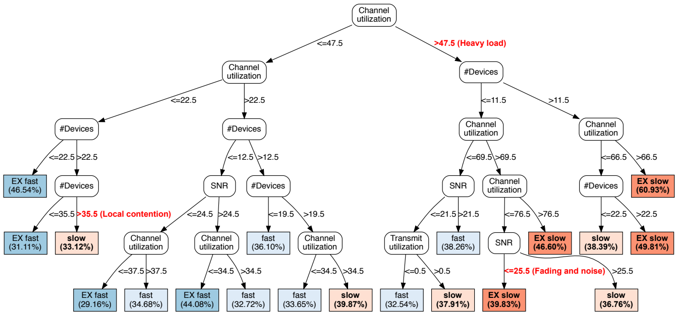
Figure 10: Decision tree for modeling the effects of radio factors on WiFi latency. The percent of the major class in the node is shown.
